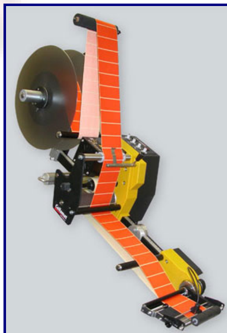
7610 High-Speed Applicator
